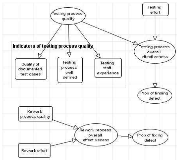
Figure 5 Testing and Rework Subnet
