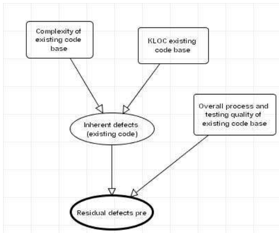
Figure 10 Stub Phase for Existing Code
