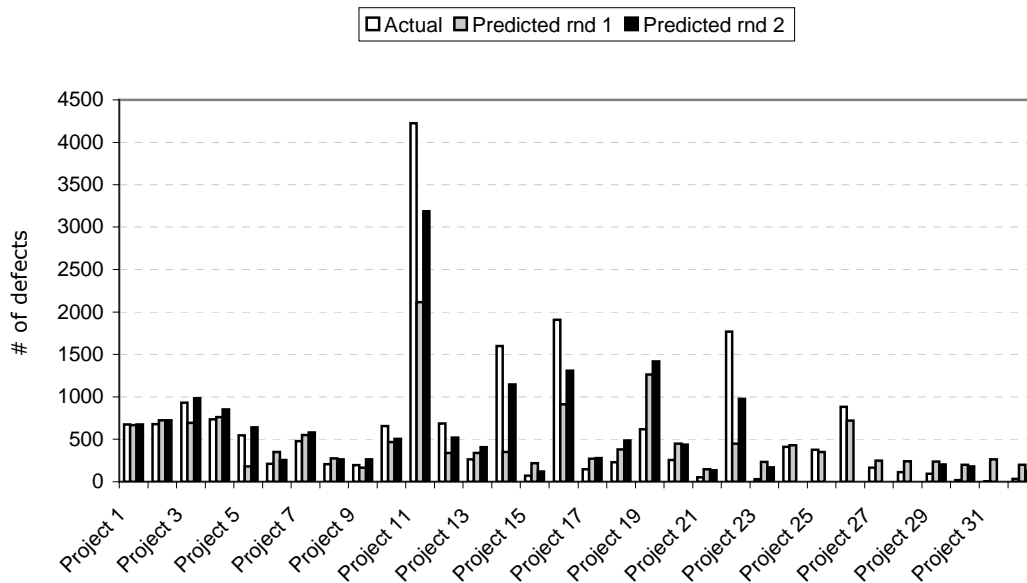
Figure 9 Accuracy of the Prediction for 32 Projects
