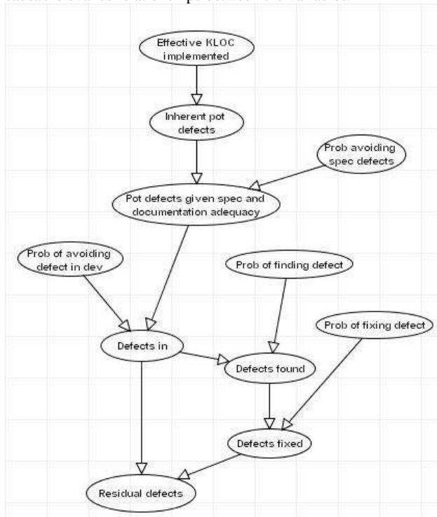
Figure 1 BN for Defect Prediction
