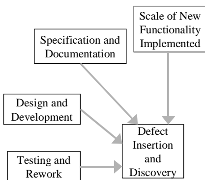
Figure 3 Subnets of the Phase BN
