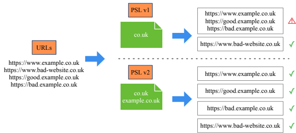
Figure 1: Illustrative example of the impact of an out-of-date Public Suffix List.
