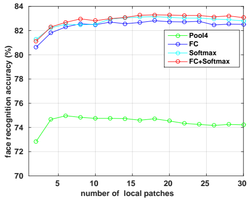
Figure 2. The performance of C-Fusion
