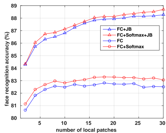
Figure 6. Face recognition accuracy using Joint Bayesian method
