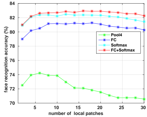
Figure 3. The performance of A-Fusion
