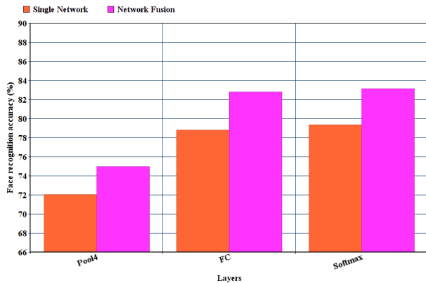
Figure 5. Comparison of single networks versus network fusion
