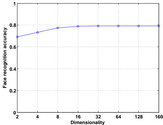
Figure 1. The impact of feature dimensionality in PCA space on face recognition rate.
