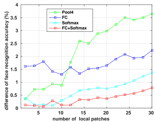
Figure 4. The accuracy margin of C-Fusion over A-Fusion.
