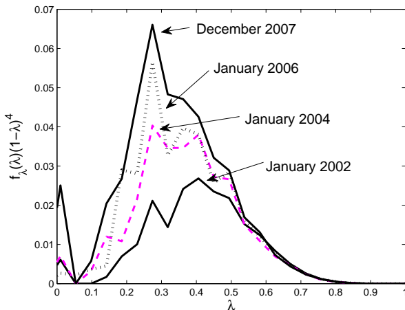
Fig. 13. Weighted Spectra Distribution, Skitter AS topology.
