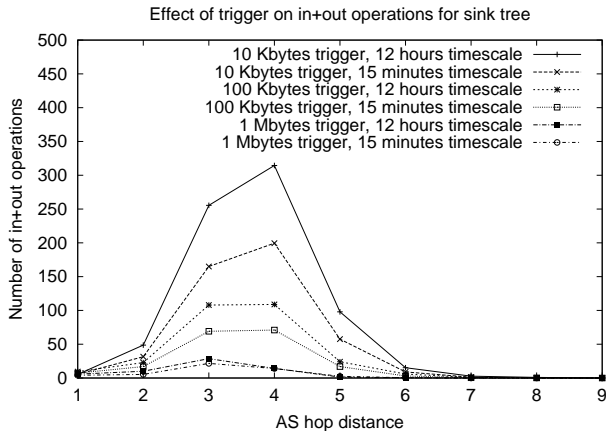
Figure 12: Effect of a trigger on in+out operations for sink tree.
