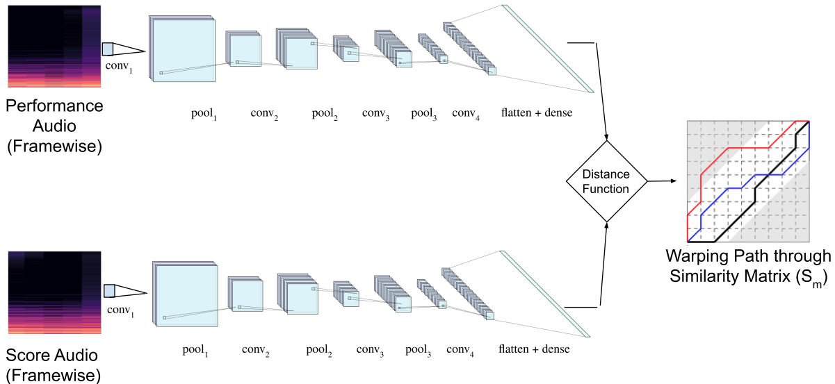
Fig. 1: Model Pipeline
