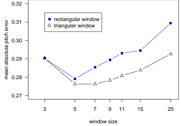
Figure 2: Pitch error (MAPE) for different sliding windows.
