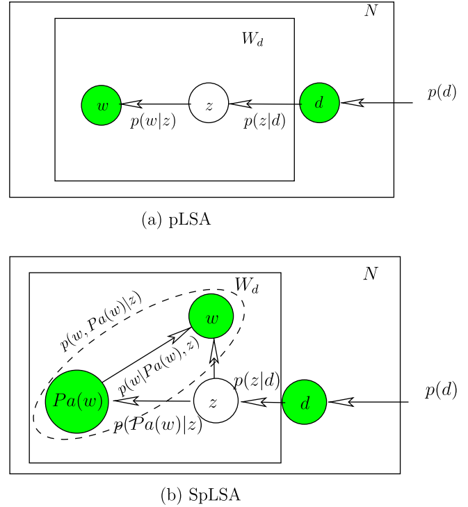
Fig. 1. Graph models of the pLSA (a) and SpLSA (b) respectively. Nodes are random variables. Filled nodes are observed and white ones are hidden. Arrows represent the dependencies between nodes. In (b), the joint probability p(w, Pa(w)|z) can be written in terms of a product: p(w|Pa(w), z)p(Pa(w)|z) .
