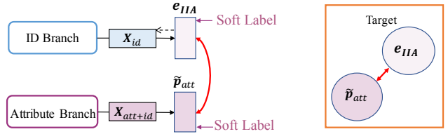
(b) Target domain adaptation of TJ-AIDL by attribute consistency
