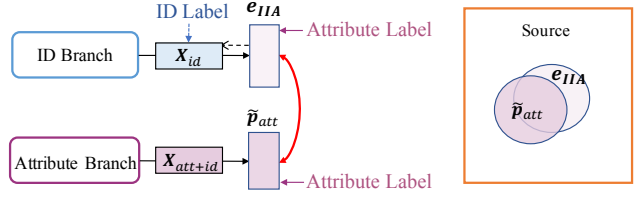
(a) Source data supervised learning of TJ-AIDL by attribute consistency
