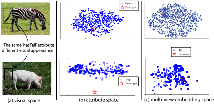
Fig. 1. Illustrating projection domain shift problem. Zero-shot prototypes are annotated as red stars and predicted semantic attribute projections shown in blue. Both Pig and Zebra share the same ‘hasTail’ attribute yet with very different visual appearance of ‘Tail’. The figure comes from [115].
