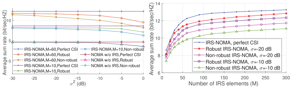
(a) Comparison between NOMA and IRS-NOMA. (b) IRS-NOMA in different levels of channel uncertainty.
