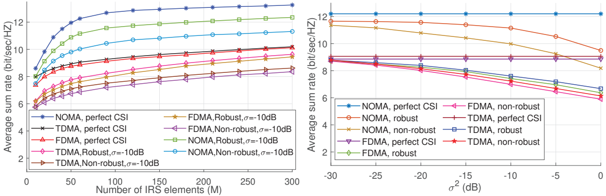
(a) Comparison in terms of Number of IRS elements.
