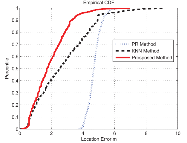
Fig. 5. Location error CDFs with \sigma = 5 dB.
