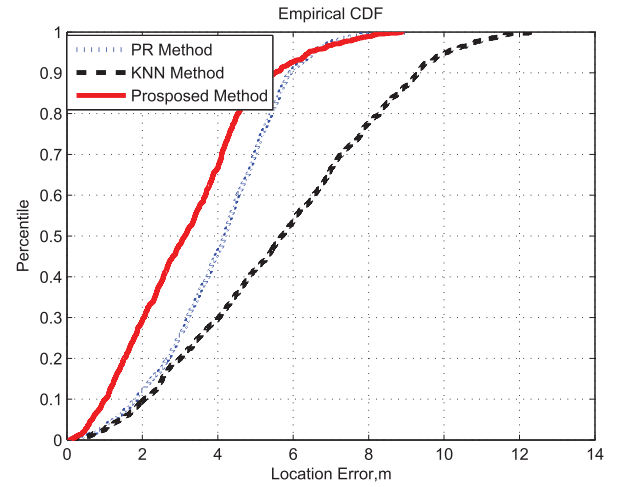
Fig. 6. Location error CDFs with \sigma = 7 dB.
