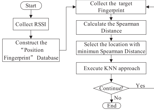
Fig. 1. Flow chart of localization.
