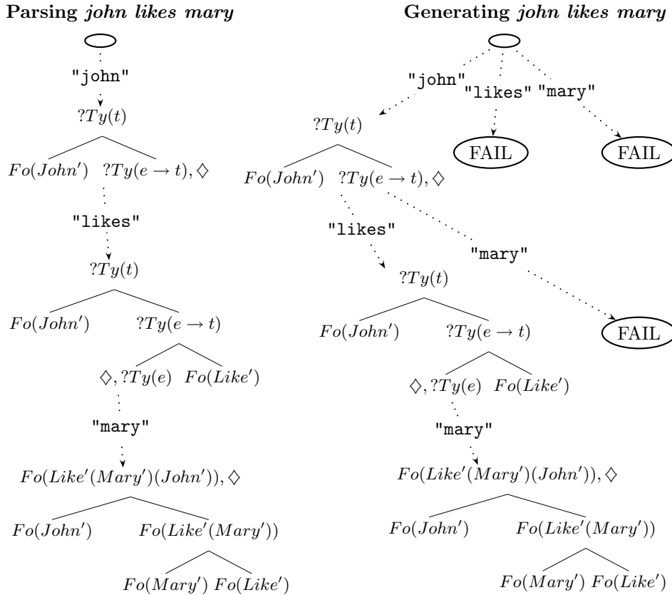
Figure 1. Parsing/generating John likes Mary
