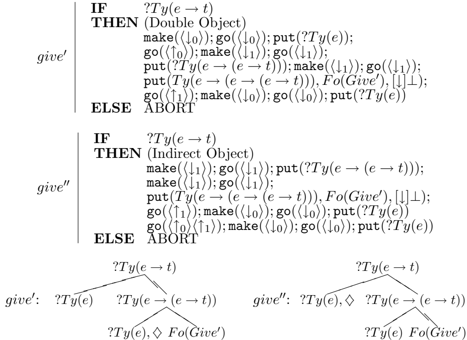
Figure 3. Output of alternative lexical actions for give
