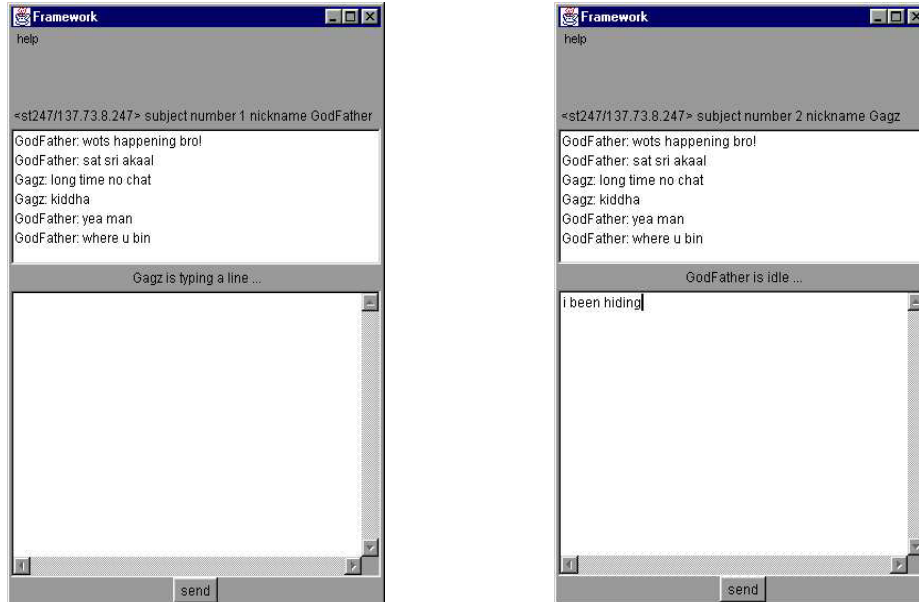
Figure 1: Chattool Client Interface
