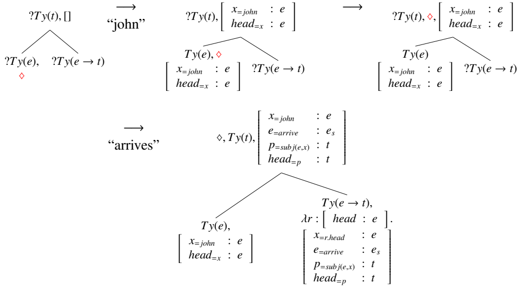
Figure 1: Incremental parsing in DS-TTR: “John arrives”
