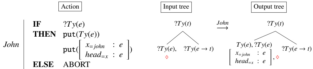
Figure 2: Lexical action for the word ‘John’
