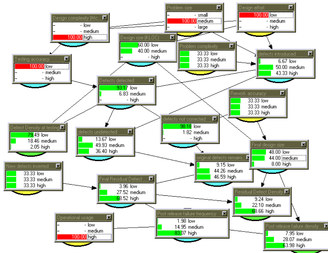
Figure 2: Entering evidence into the BBN – an explanation for the ‘paradox’ of low defect density pre-release but high defect density post-release
