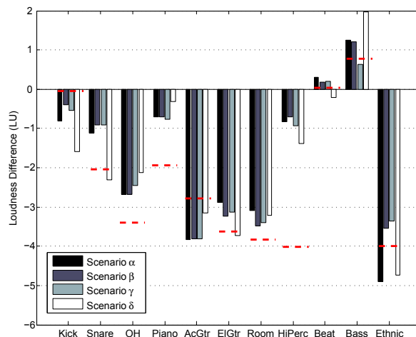
Fig. 5: New results referenced to vocals. The dashed horizontal lines represent the old results, and the four bars show how the scenarios presented in the text could improve the algorithm's agreement with the evaluation data.
