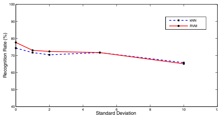
Fig. 5. Overall recognition rate, with respect to the sigma of the Gaussian noise that was added to the saliency values of the detected salient points prior to clustering.
