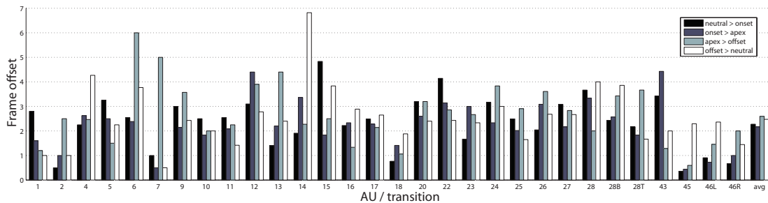
Fig. 15: Average detection offsets per AU and temporal segment transition.
