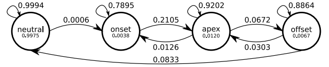
Fig. 12: The states and transition probabilities for an HMM trained on AU 1. Initial probabilities are denoted below the state names. Transitions with probability 0 are not shown.
