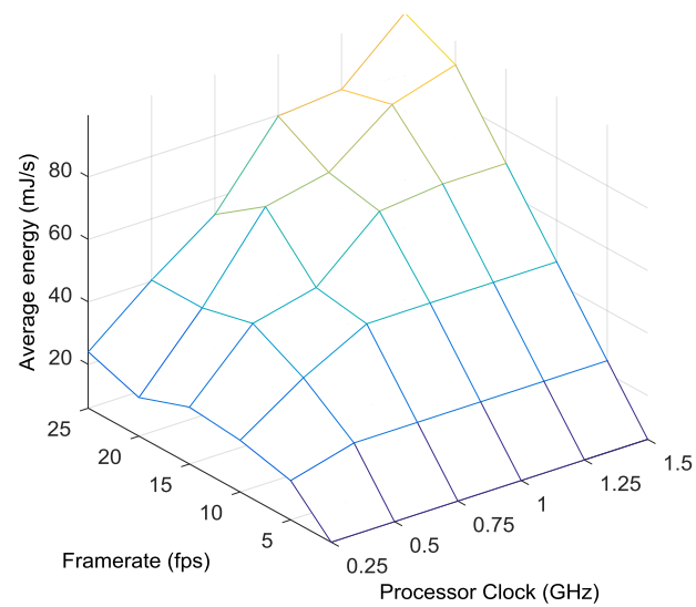
Overall energy consumption of communication
