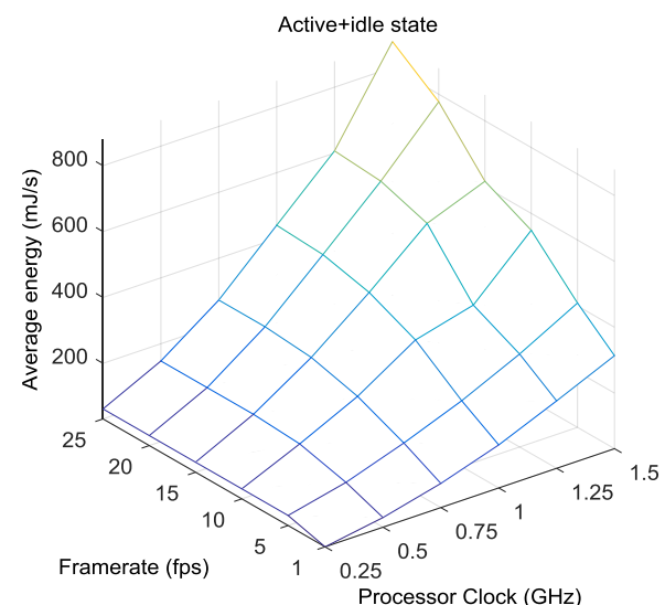
Energy consumption of processing (overall, active and idle states)
