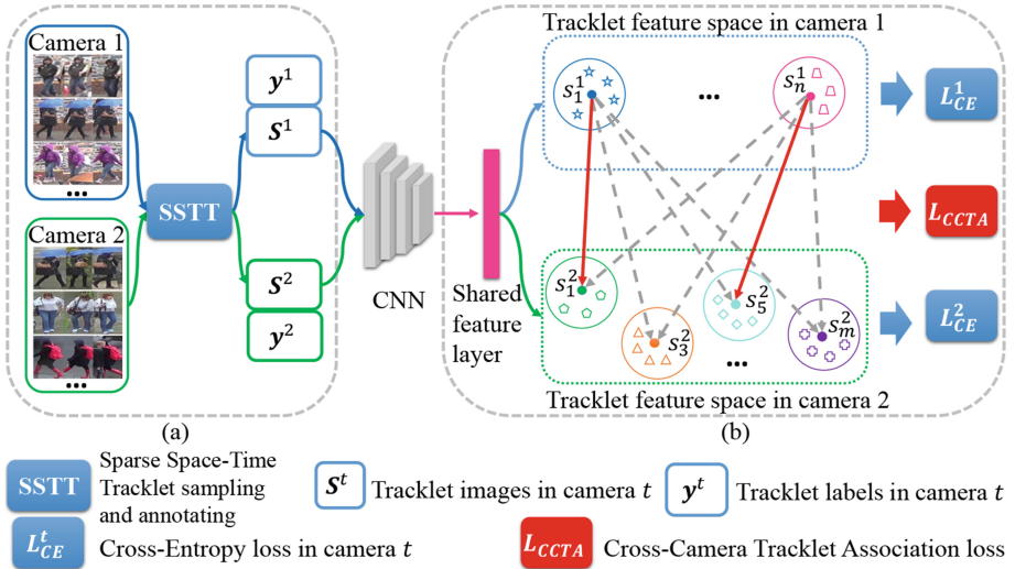
Fig. 1. An overview of Tracklet Association Unsupervised Deep Learning (TAUDL) re-id model: (a) Per-camera unsupervised tracklet sampling and label assignment; (b) Joint learning of both within-camera tracklet discrimination and cross-camera tracklet association in an end-to-end global deep learning on tracklets from all the cameras.
