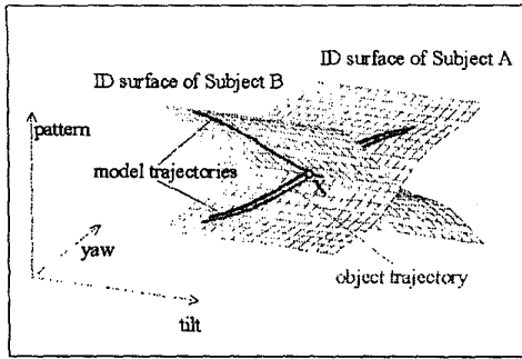
Figure 3. Identity surfaces.
