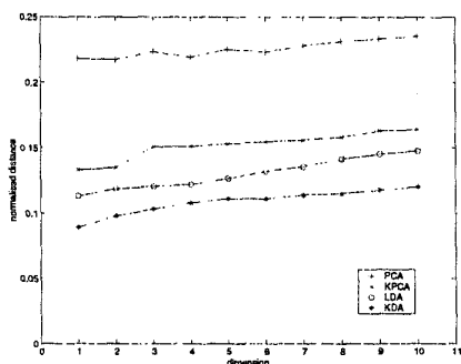
Figure 5. Recognition reliability.
