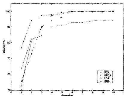
Figure 6. Recognition accuracy.
