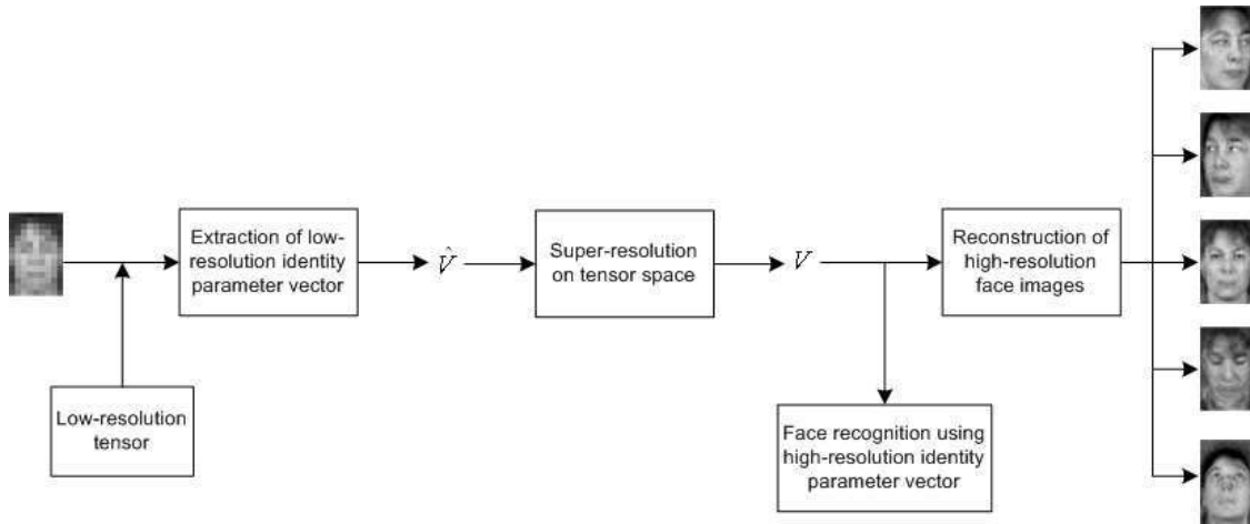
Figure 1: An illustration of our multi-modal super-resolution and recognition process in tensor space using a multi-view super-resolution example.
